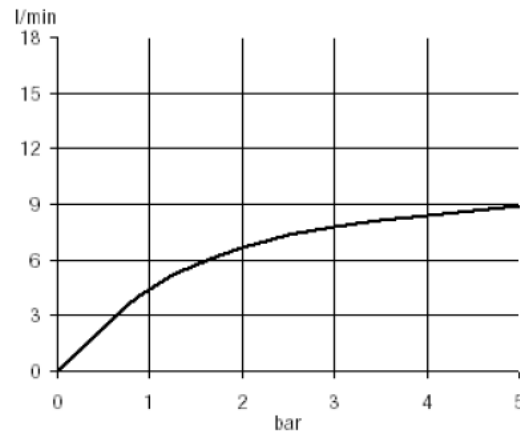
Perlator Eco S-pointer
